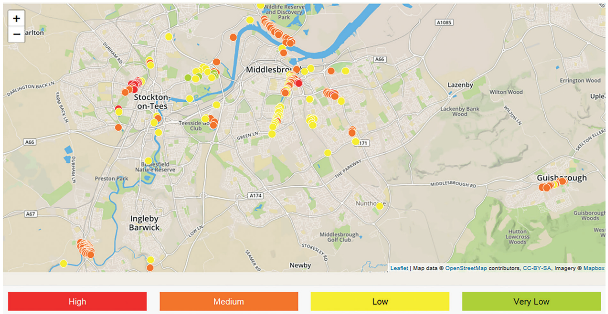
Fig. 2 – Flood risk map for Middlesbrough
